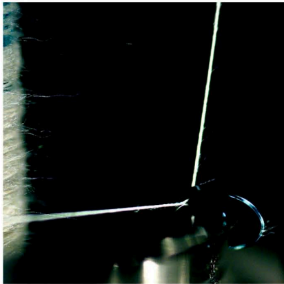
RZD PROTECTED RINGS DURING SPINNING PROCESS
